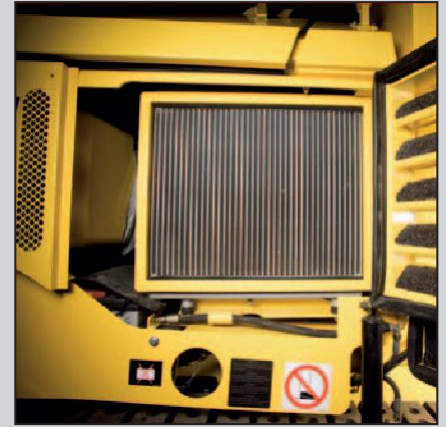
The engine compartment is accessible from three sides. This shows the generously dimensioned cooler.
